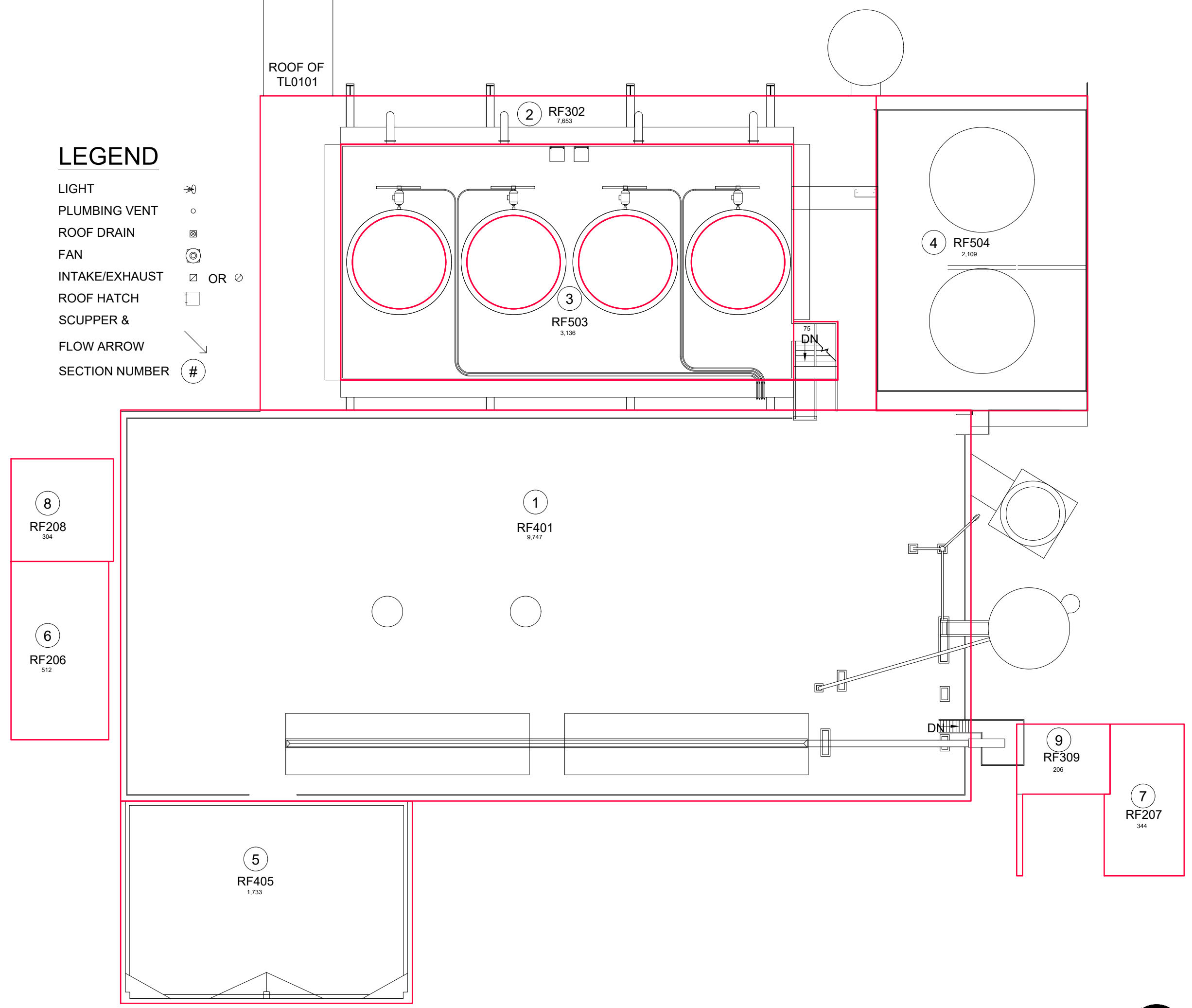
ROOF PLAN MEDICAL CENTER HEATING AND COOLING PLANT
