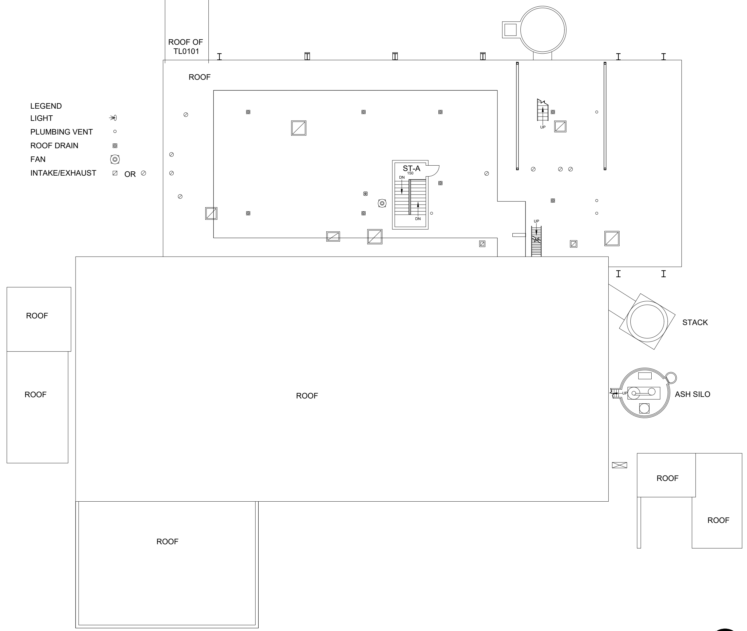
THIRD FLOOR PLAN MEDICAL CENTER HEATING AND COOLING PLANT 185 Gross Square Ft.
