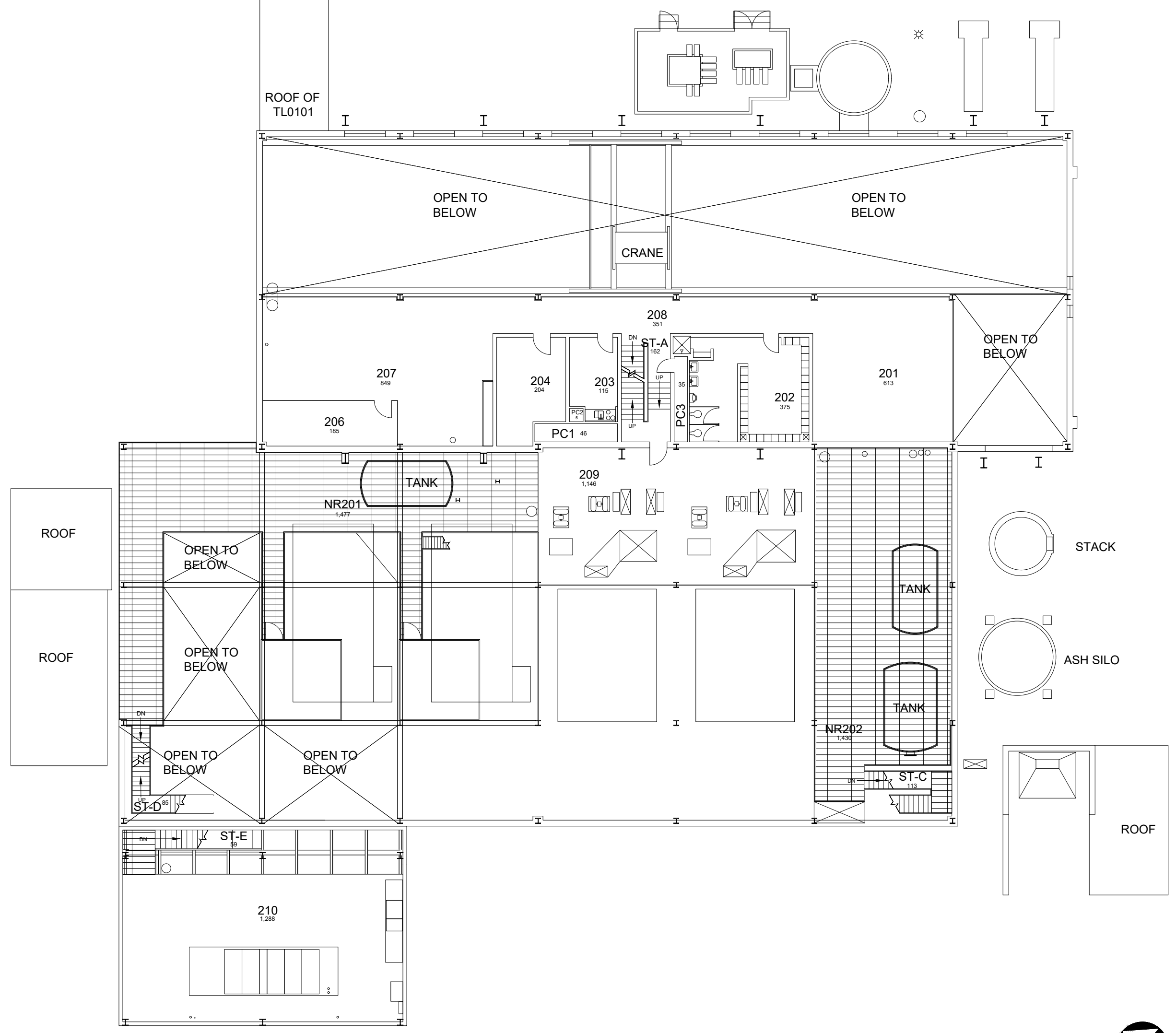
SECOND FLOOR MEZZANINE MEDICAL CENTER HEATING AND COOLING PLANT 9,396 Gross Square Ft
