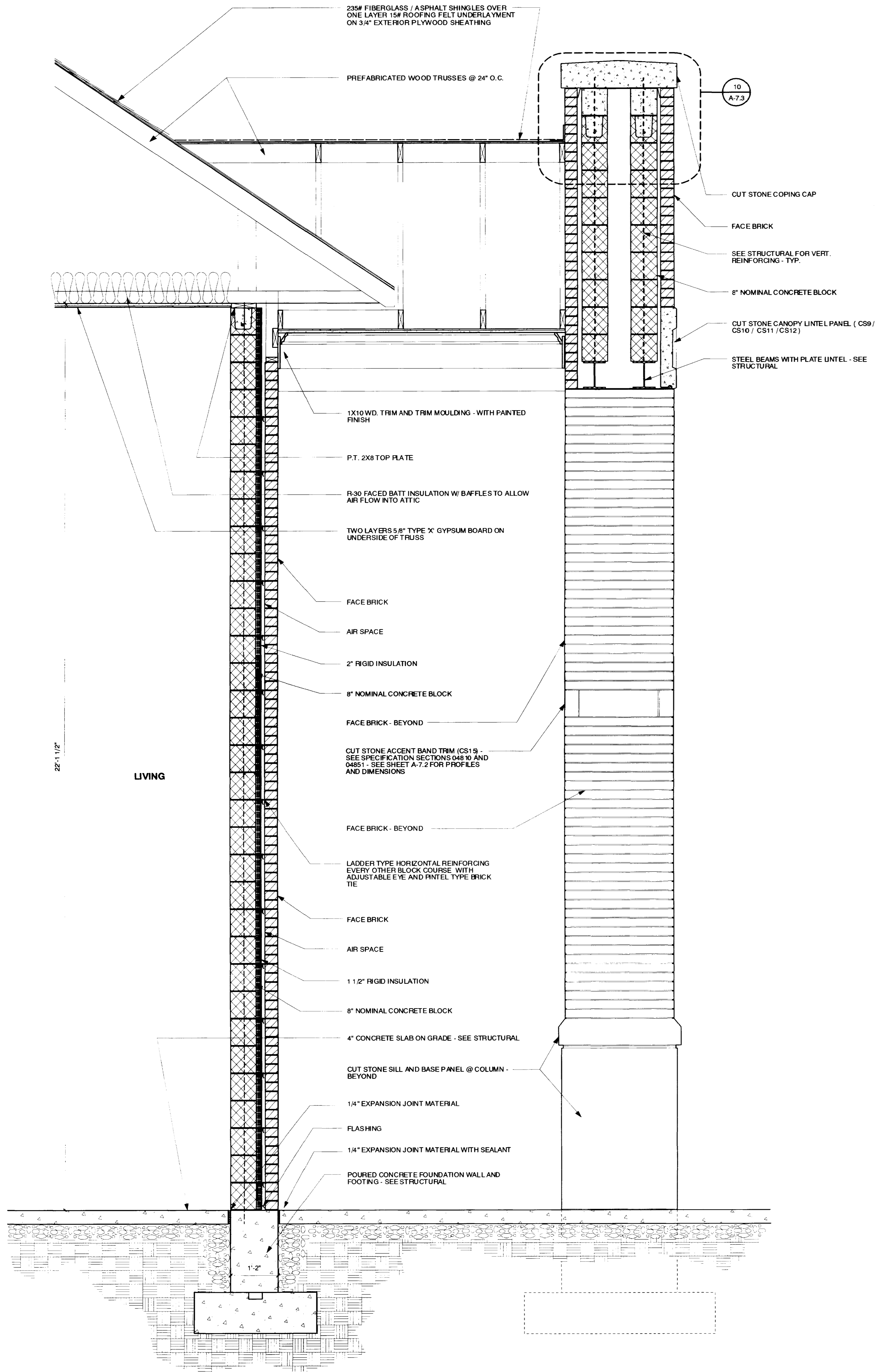
1 WALL SECTION 3/4" = 1'-0"
