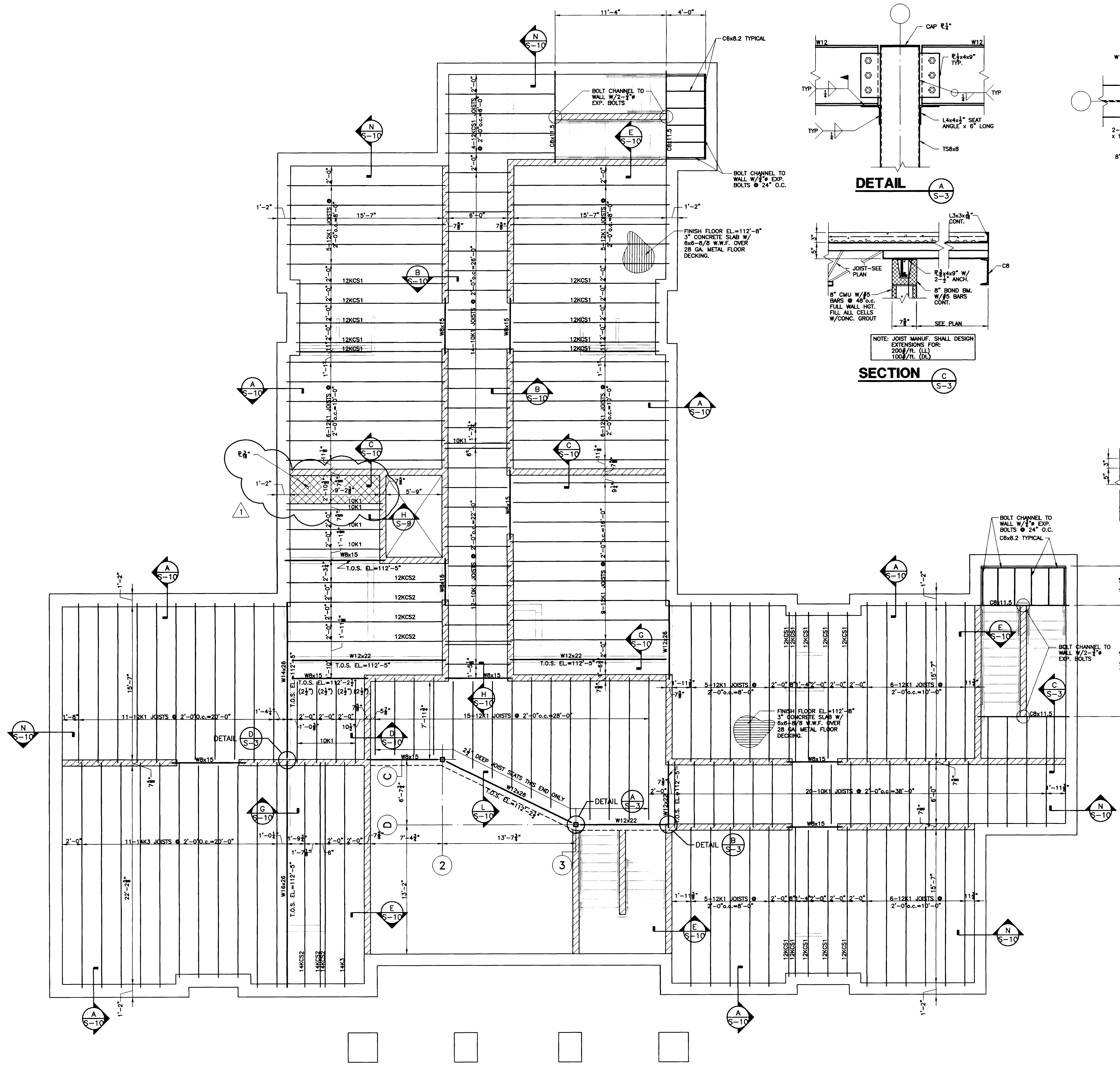
SECOND FLOOR FRAMING PLAN - BUILDING 0504 (NOTE: ALL JOISTS THIS SHEET SHALL HAVE 5" DEEP BEARING SEATS U.N.O.) (JOISTS BEARING EL.=112'-0")
