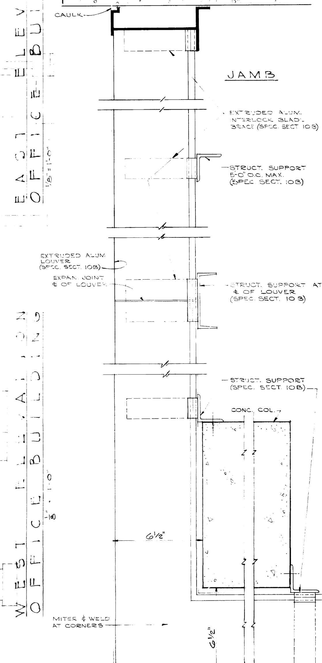
SECTION A-A SECTION B-B WEST ELEVATION EAST ELEVATION OFFICE BUILDING
