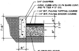
CURB DETAIL NO SCALE
