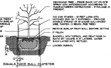
TREE DETAIL NO SCALE
