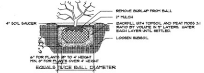
SHRUB DETAIL NO SCALE
