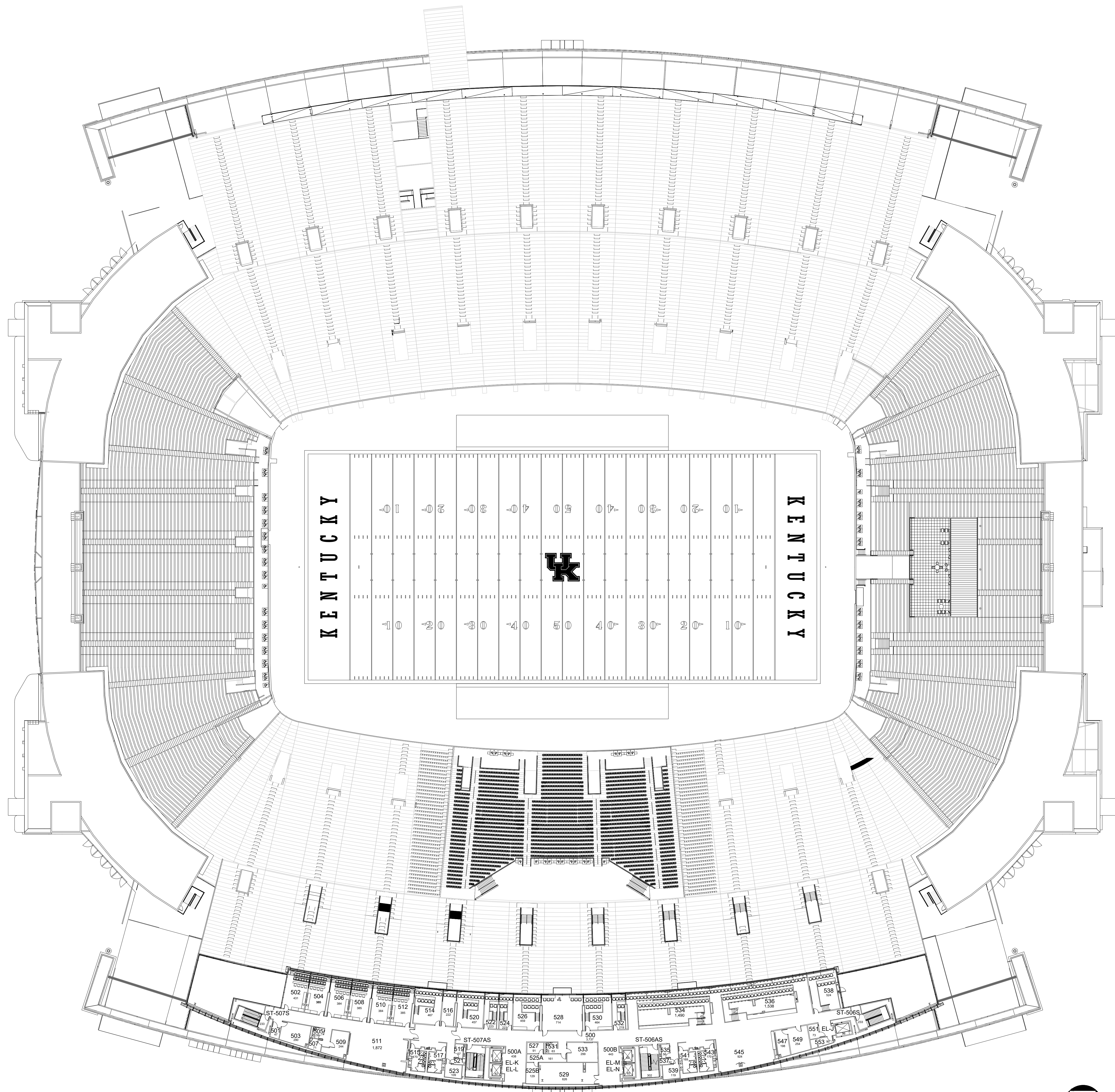
PRESS LEVEL PLAN KROGER FIELD 25,824 Gross Square Ft.
