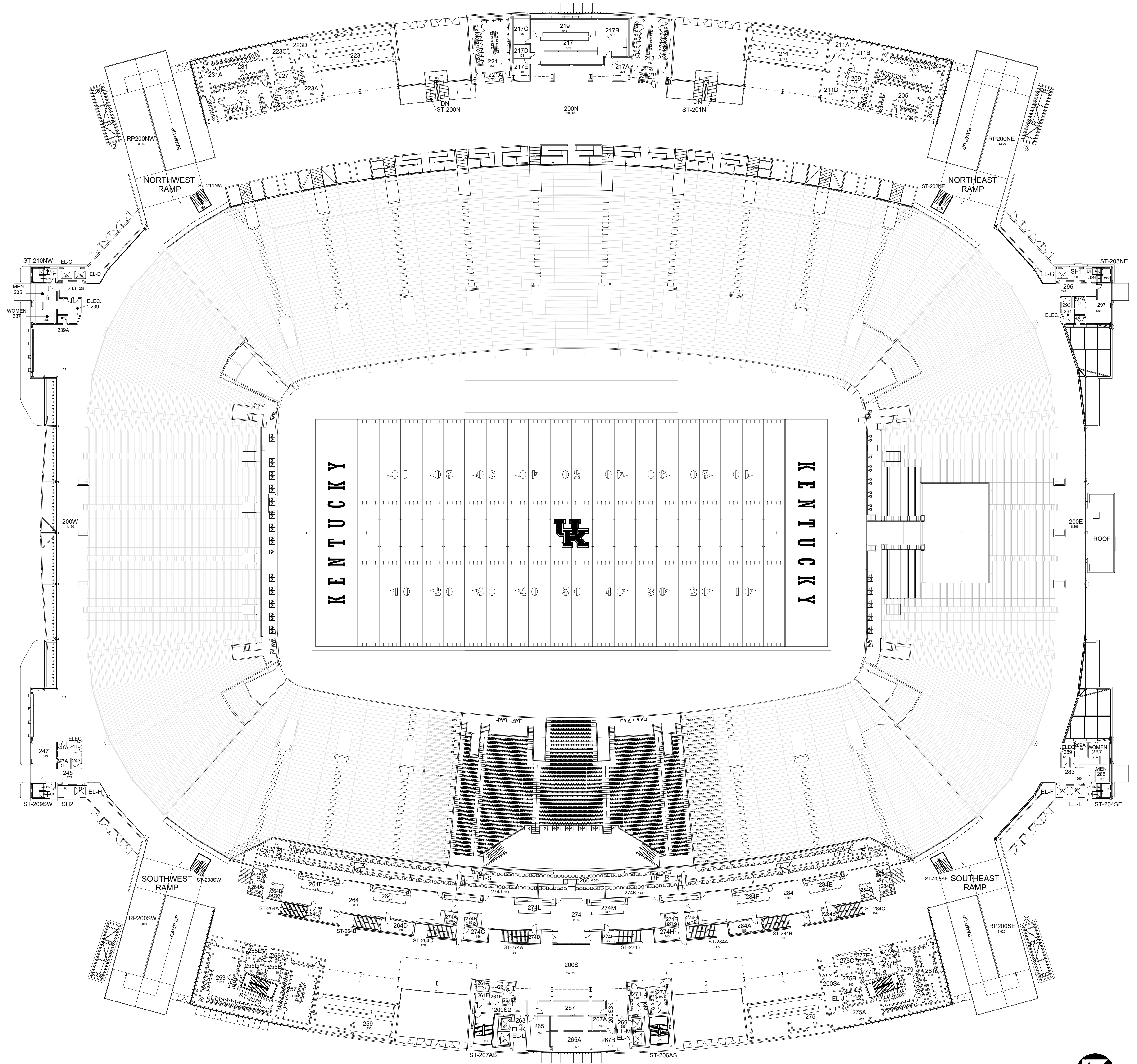
UPPER CONCOURSE LEVEL PLAN KROGER FIELD 171,922 Gross Square Ft.
