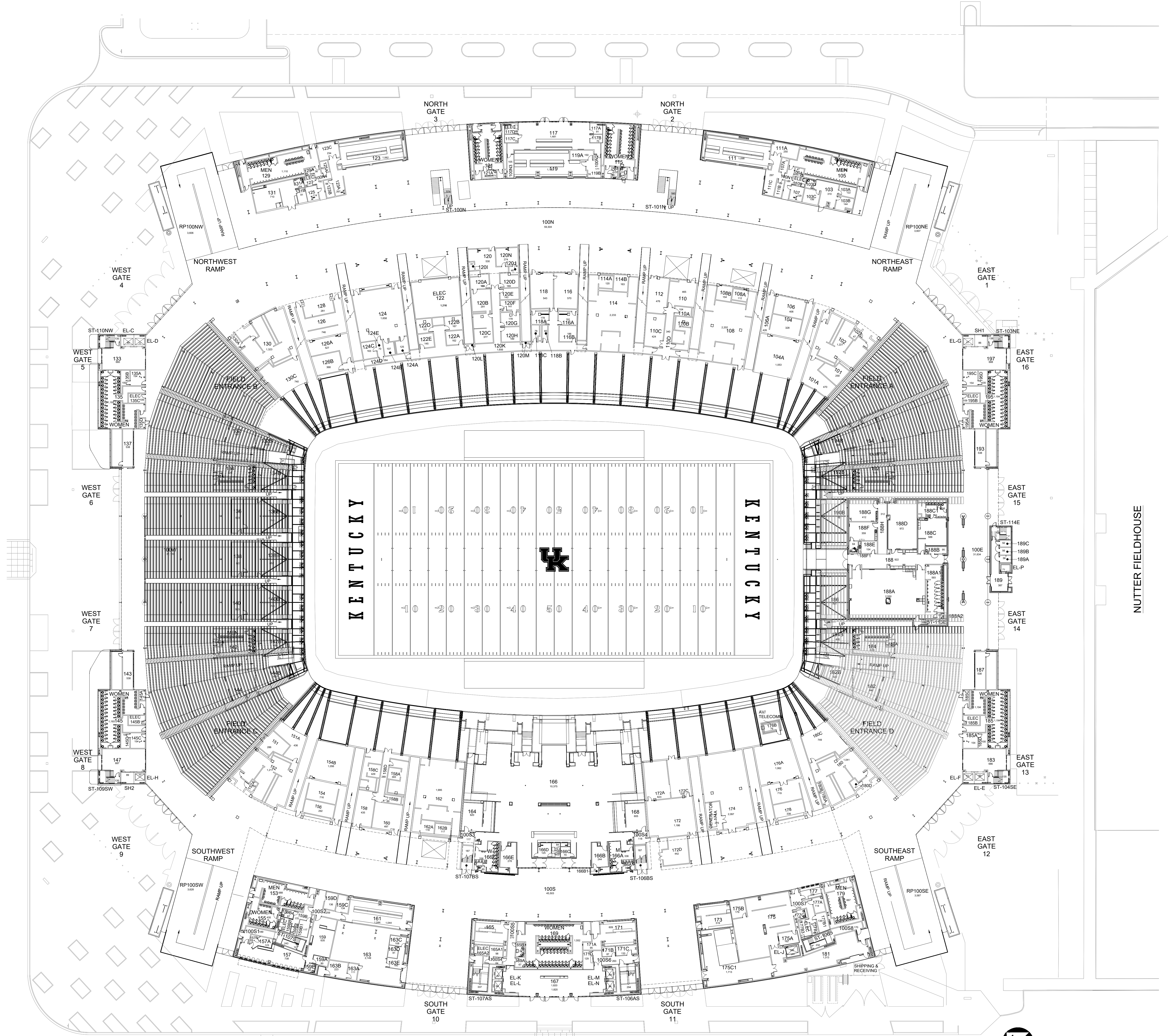
LEVEL 1 - MAIN CONCOURSE LEVEL PLAN KROGER FIELD
