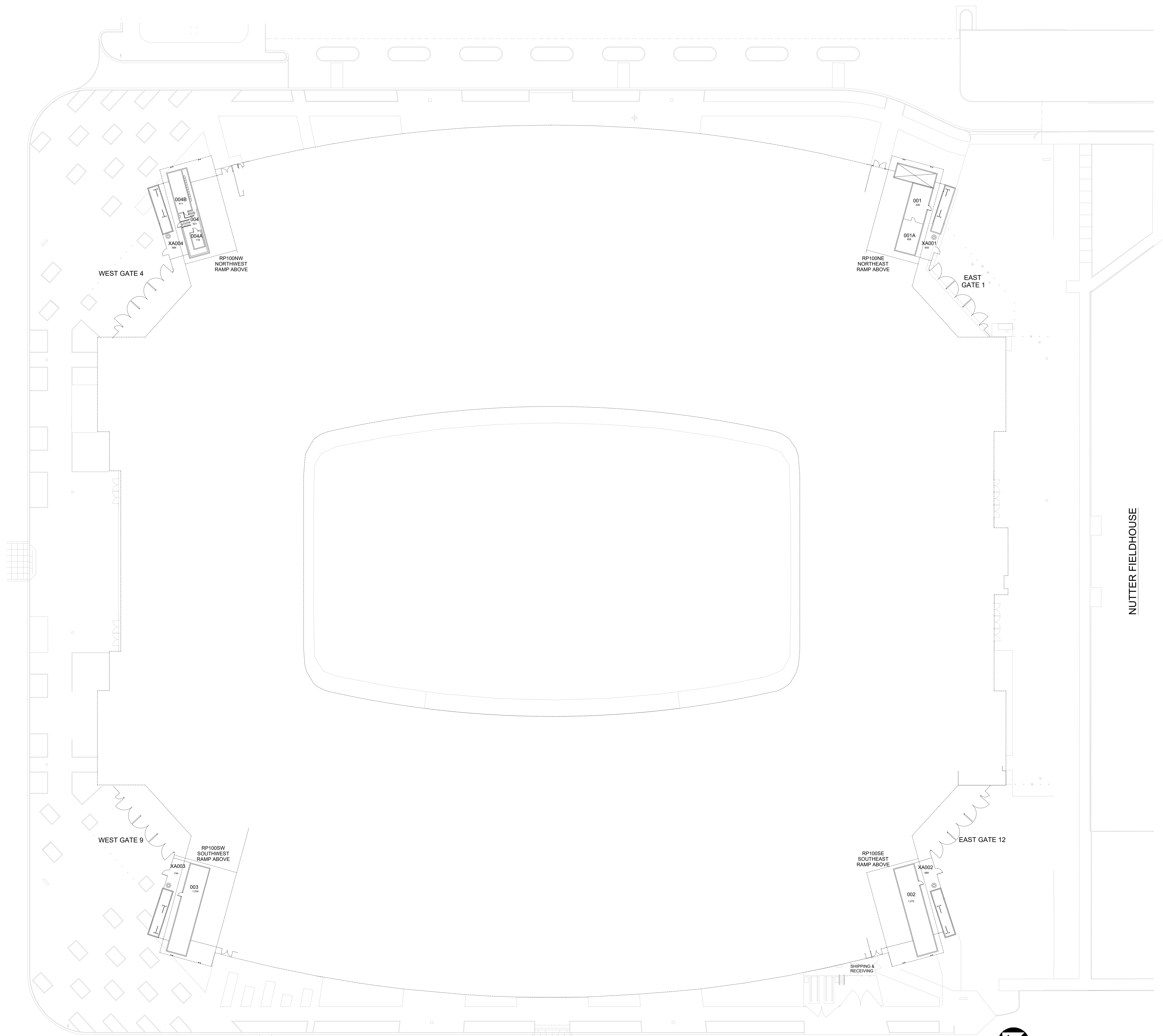
LEVEL 0 - BELOW MAIN RAMPS PLAN KROGER FIELD 7,910 Gross Square Ft.
